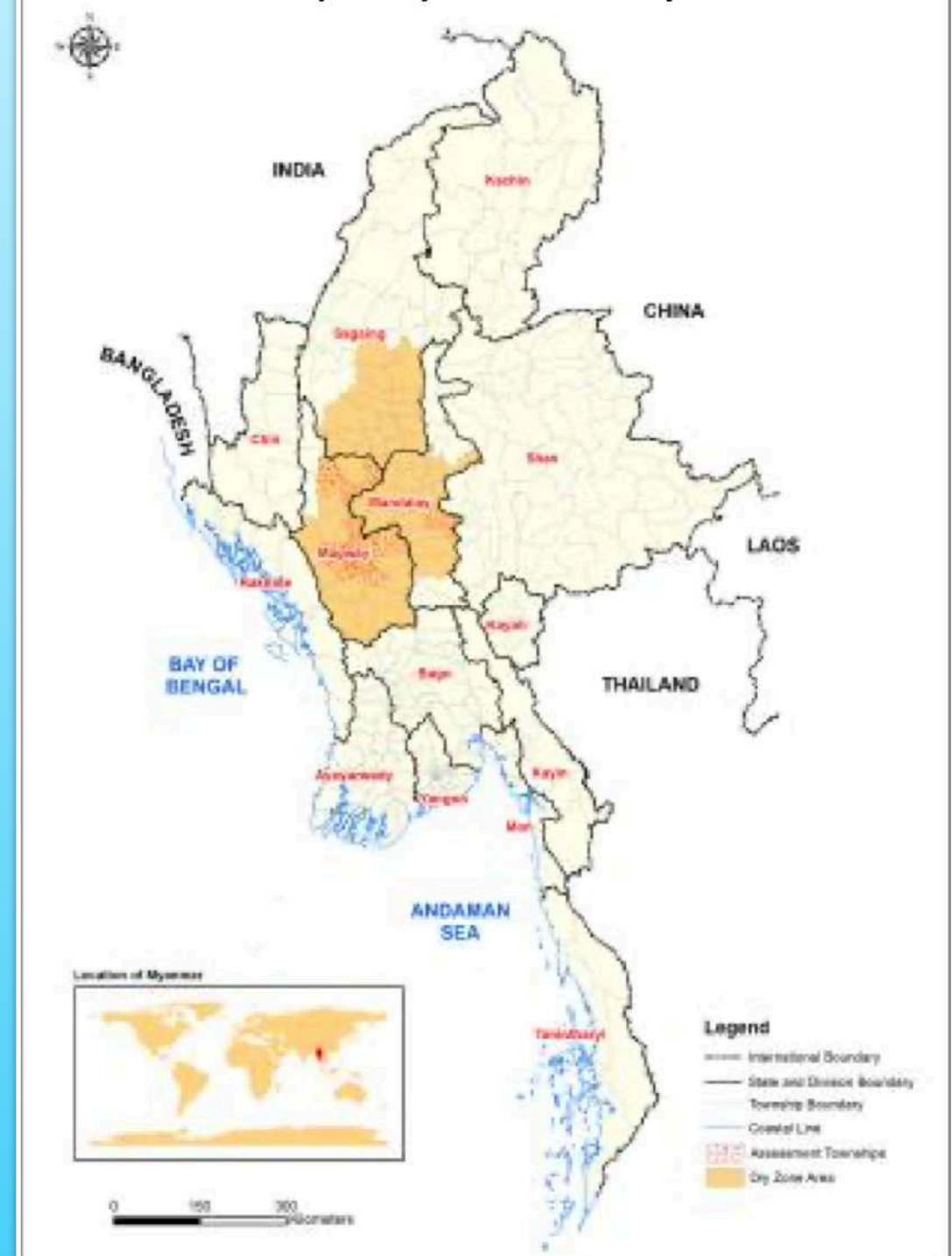
Map 1: Dry Zone within Myanmar
